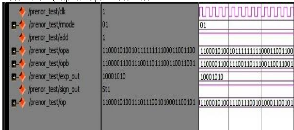
Fig. 9 Addition / subtraction results with the IEEE 754 numbers
