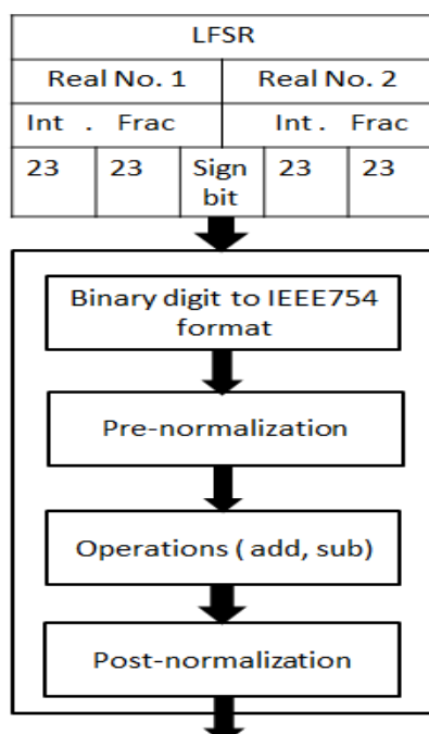
Fig. 2 FPAU design and operation flow
