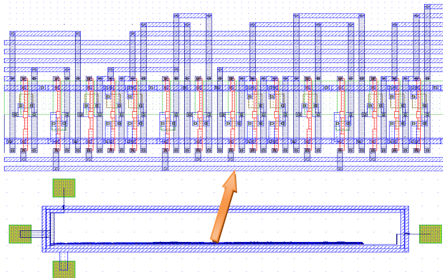
Fig. 7 90nm Technology LFSR Test Sequence Generator
