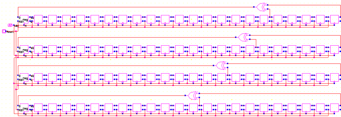
Fig. 6 Cell level LFSR design
